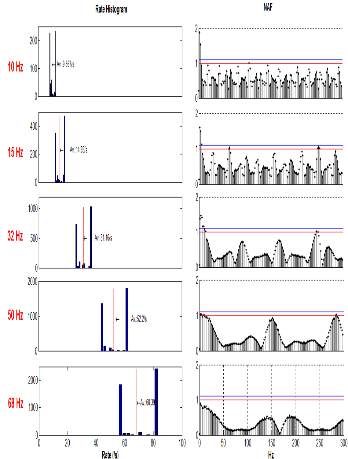
Figure 3.2: RAD sequences at rates of 10, 15, 32, 50 and 68 Hz showing (Left column), the rate histograms and (Right column), the noise amplification factors (NAF).
