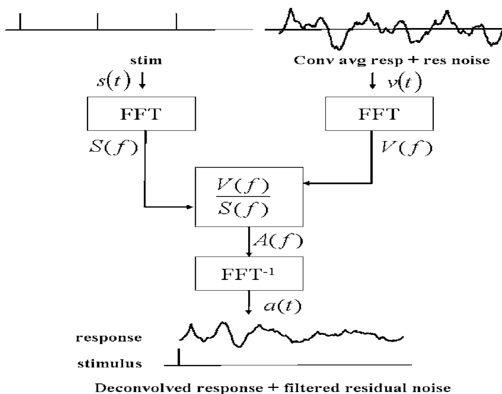
Figure 2.14: The convolution of the responses and sequence stimulus to the frequency domain to extract the per-stimulus response (Ozdamar & Bohorquez 2006).
